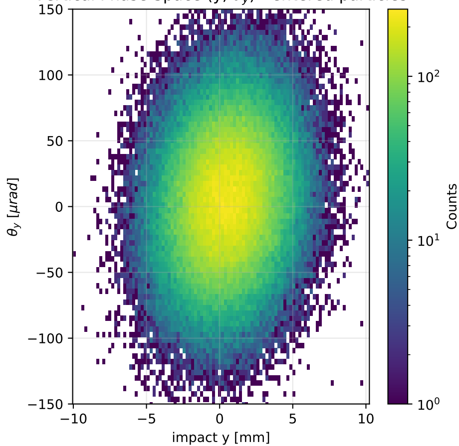
Vertical Phase Space (y, \theta_y ) - entered particles
