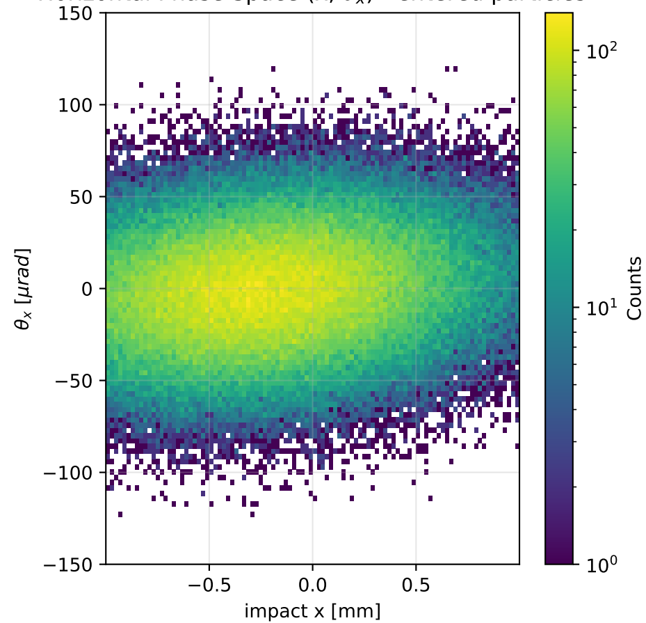
Horizontal Phase Space (x, \theta_x ) - entered particles
